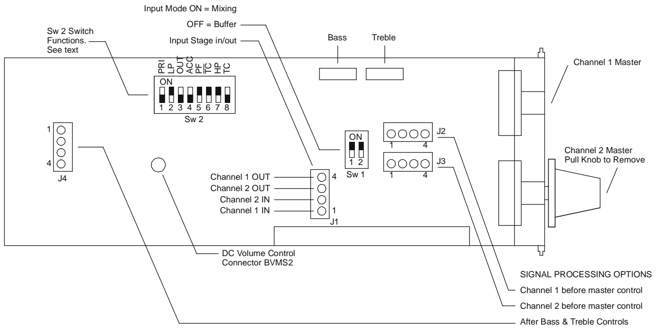
Fig 1: BVMS1 Connector and Switch Locations
